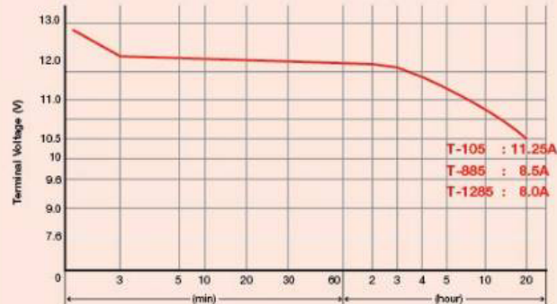
T-105, T-885, T-1285 Discharged
